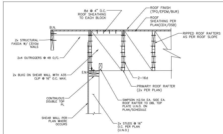
SIDE END OF THE RAFTER
