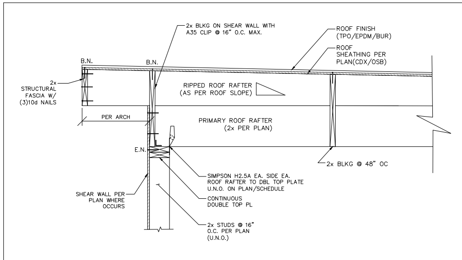
FRONT END OF THE RAFTER
