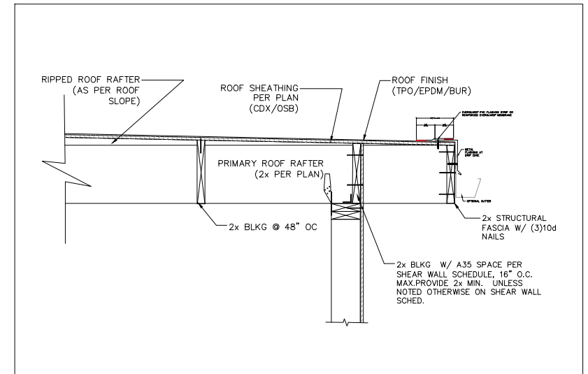
REAR END OF THE RAFTER
